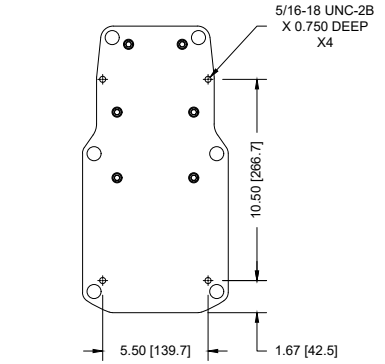
BENCH MOUNTING HOLES BOTTOM VIEW
